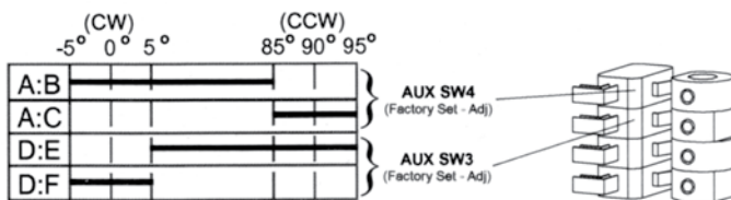
Switch/Cam arrangement for On/Off control
