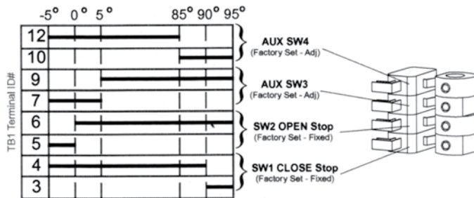
Switch/Cam arrangement for Jog & Proportional control
